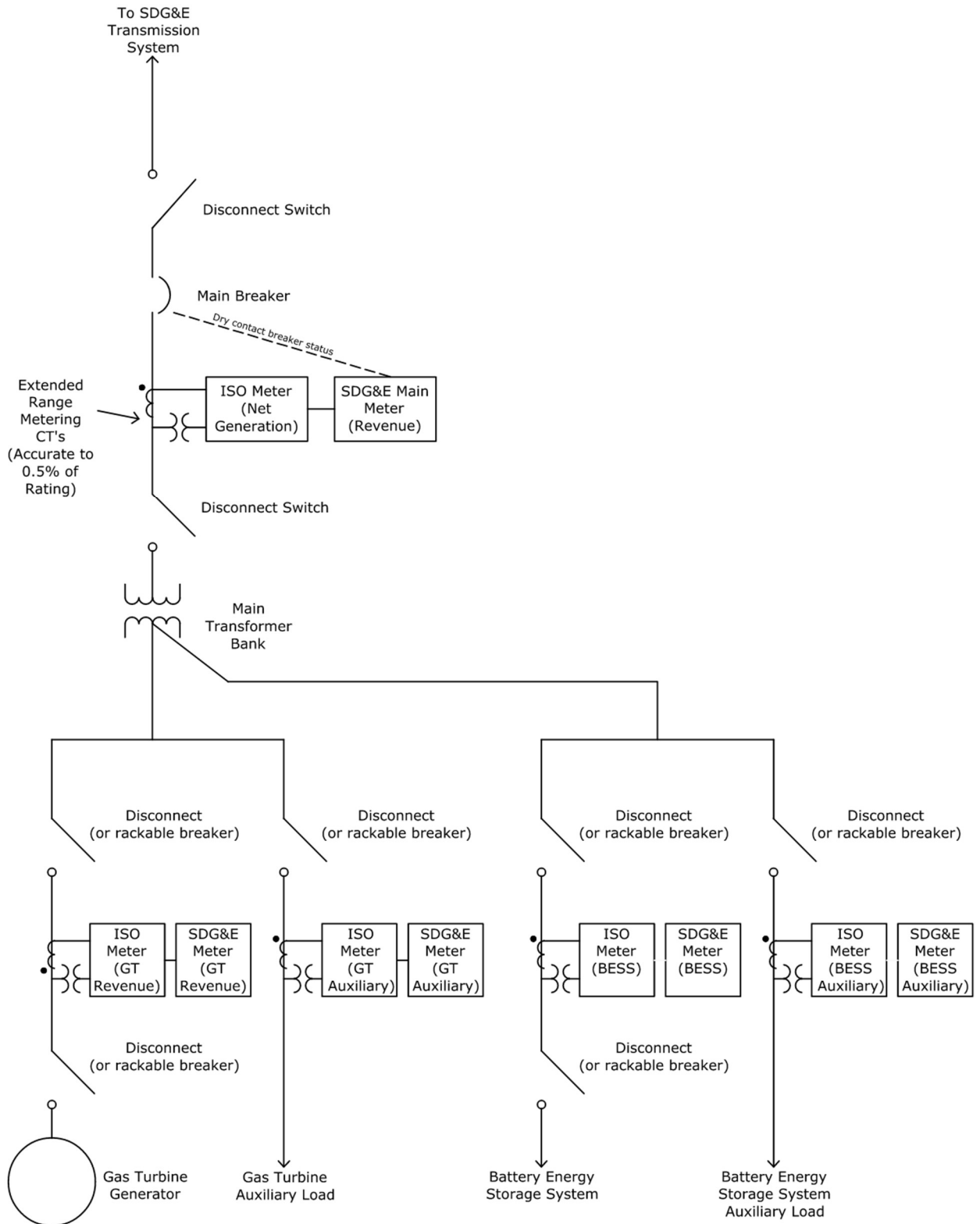
Figure 3.3 Transmission Interconnection Metering with Multiple Co-Located Resources Layout Method #3
